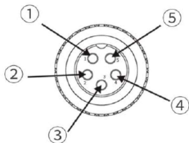
Diagram of aviation plug female port
